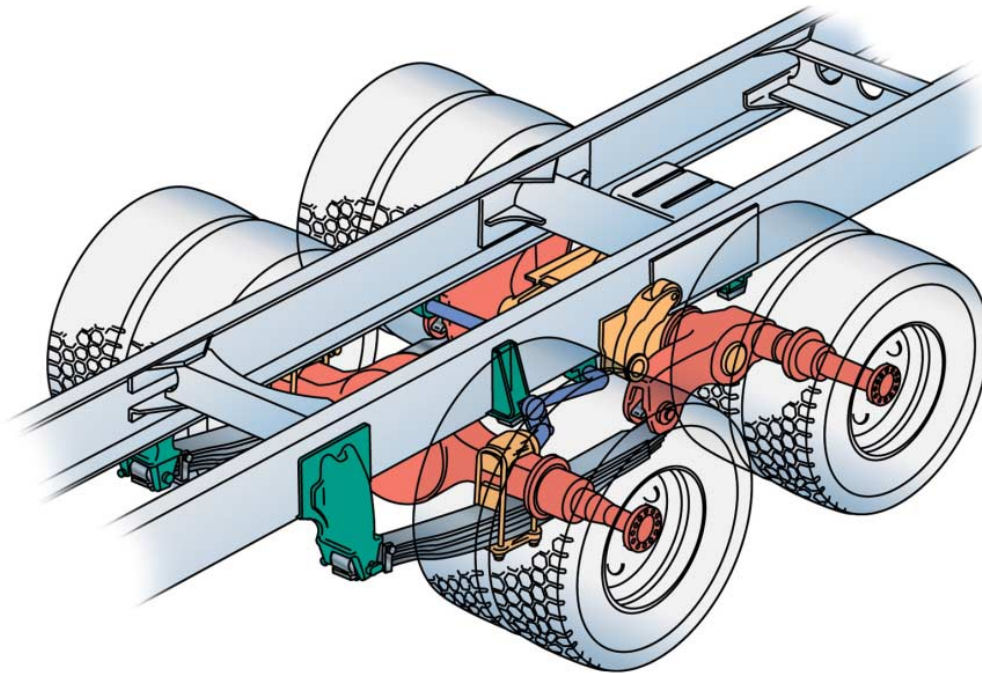
RADT-AR, leaf suspended bogie.
